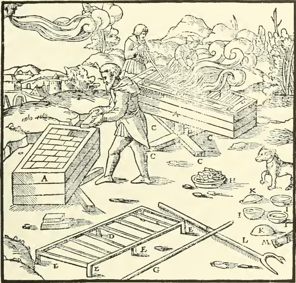
A—BOX. B—PIVOT. C—TRANSVERSE WOOD BEAMS. D—GRATE. E—ITS FEET. F—BURNING WOOD. G—STICK. H—PANS IN WHICH THE BISMUTH IS MELTED. I—PANS FOR MOULDS. K—CAKES. L—FORK. M—BRUSH.
